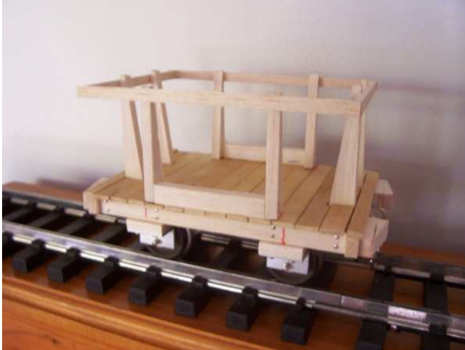
Balsa frame and decking, frame glued and pinned. Removable Skip Buckets made from Butter
